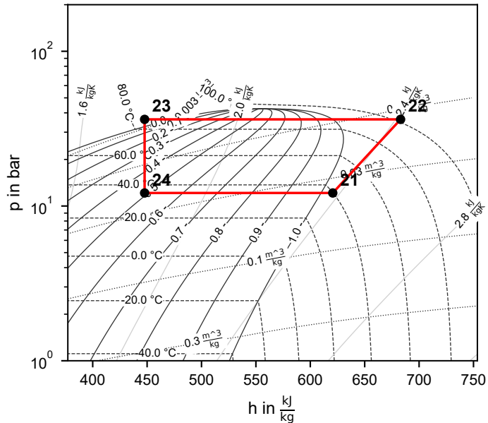
Cycle 1 (R290)
