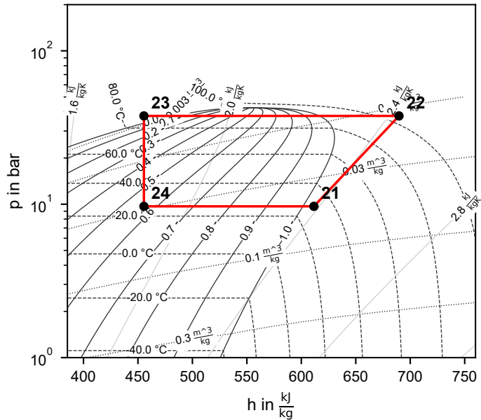
Cycle 1 (R290)
