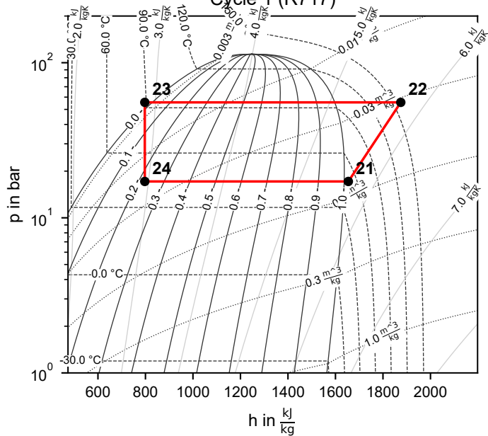
Cycle 1 (R717)
