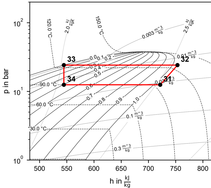
Cycle 2 (R600)
