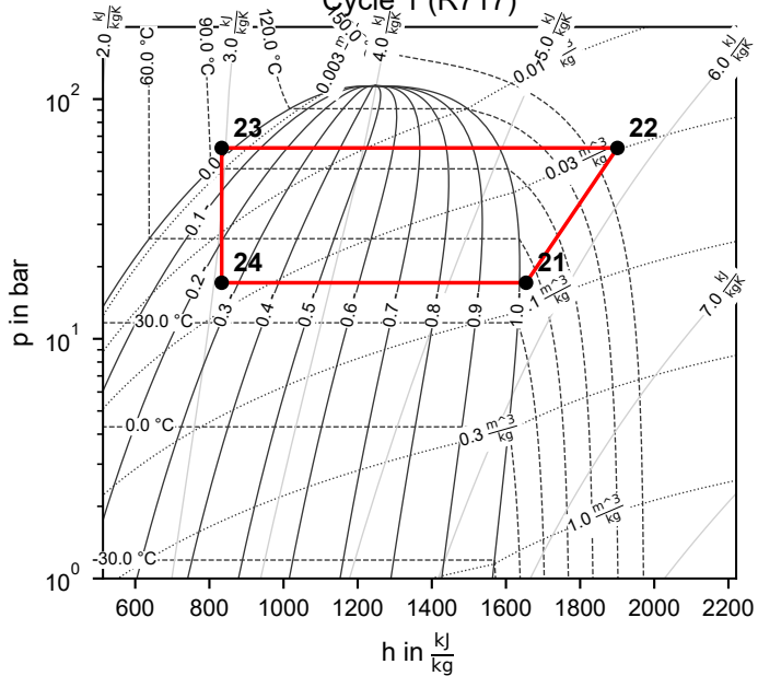
Cycle 1 (R717)
