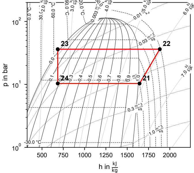
Cycle 1 (R717)
