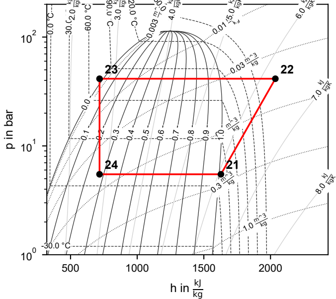
Cycle 1 (R717)
