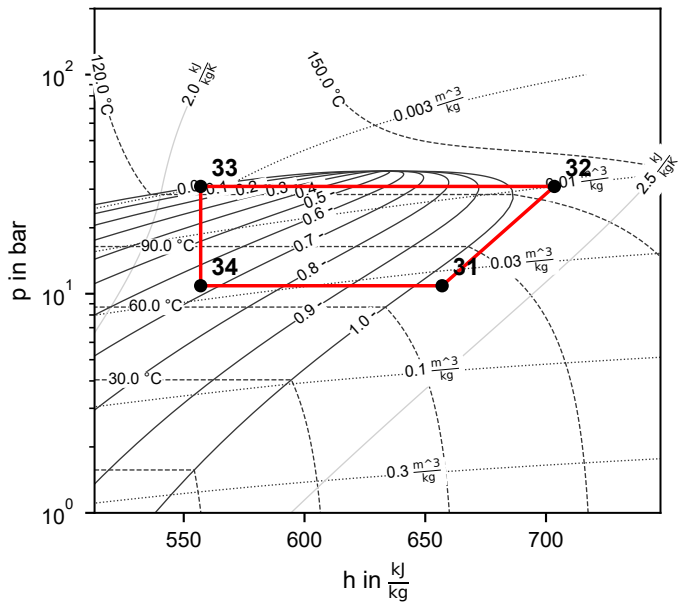
Cycle 2 (R600a)
