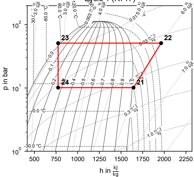
Cycle 1 (R717)
