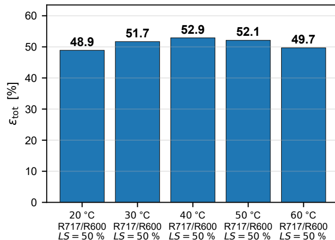
Exergetic efficiency
