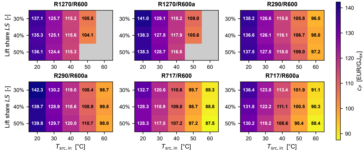
C_p heatmap per design ( T_{\text{steam}} = 100\text{ }^{\circ}\text{C} )
