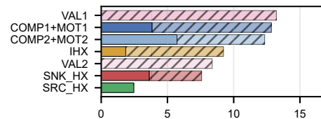
Exergoeconomic \dot{Z} + \dot{C}_D
