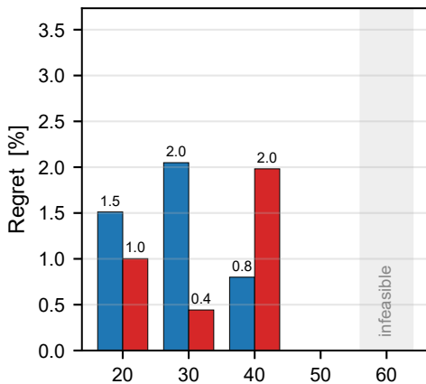
R290/R600a
