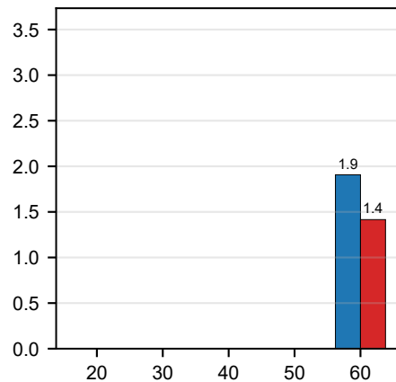
R717/R600a
