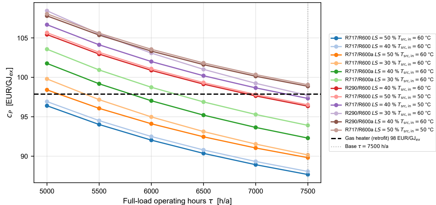
C_P vs full-load hours — 12 cheapest designs ( T_{\text{steam}} = 110\text{ }^{\circ}\text{C} )
