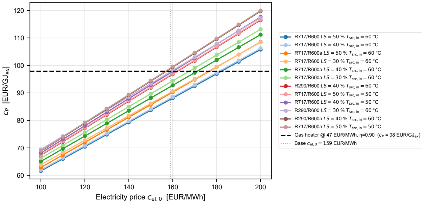
C_p vs electricity price — 12 cheapest designs ( T_{\text{steam}} = 110\text{ °C} )
