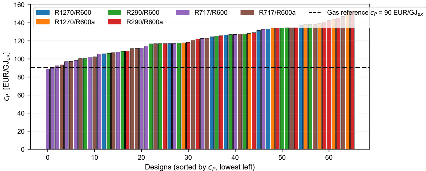
c_p — all OK designs sorted ( T_{\text{steam}} = 120\text{ °C} )
