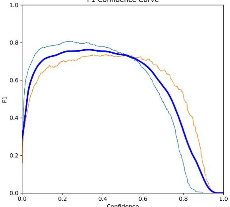
F1-Confidence Curve
