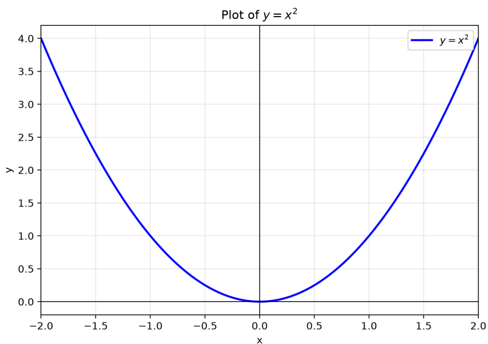
Figure 1: The graph of y = x^2 on the interval [-2, 2] .
