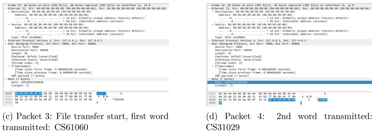
Figure 4: First four packets exchanged when the file was available.
