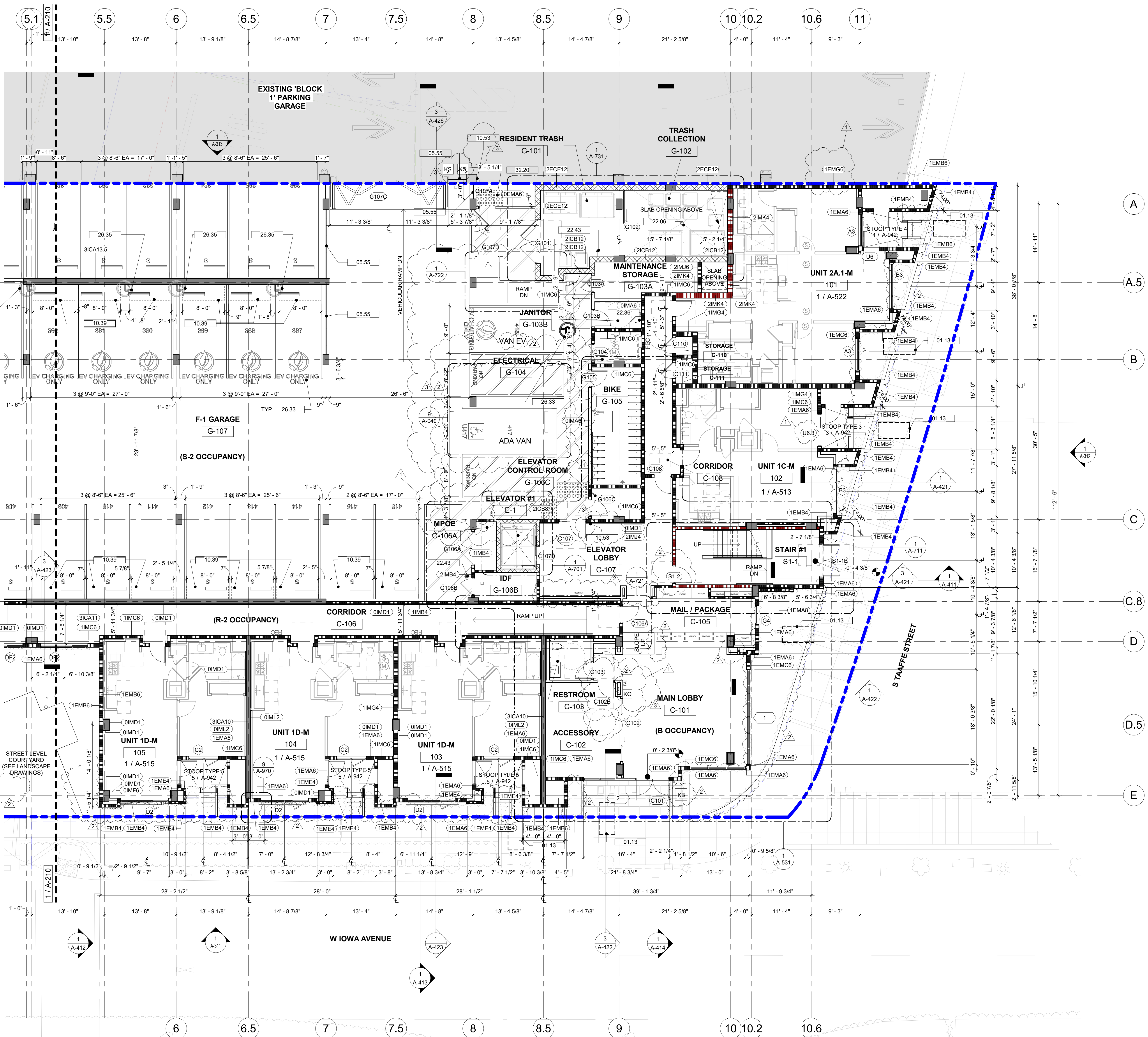
BUILDING PLAN LEVEL 1 - SEGMENT 2
