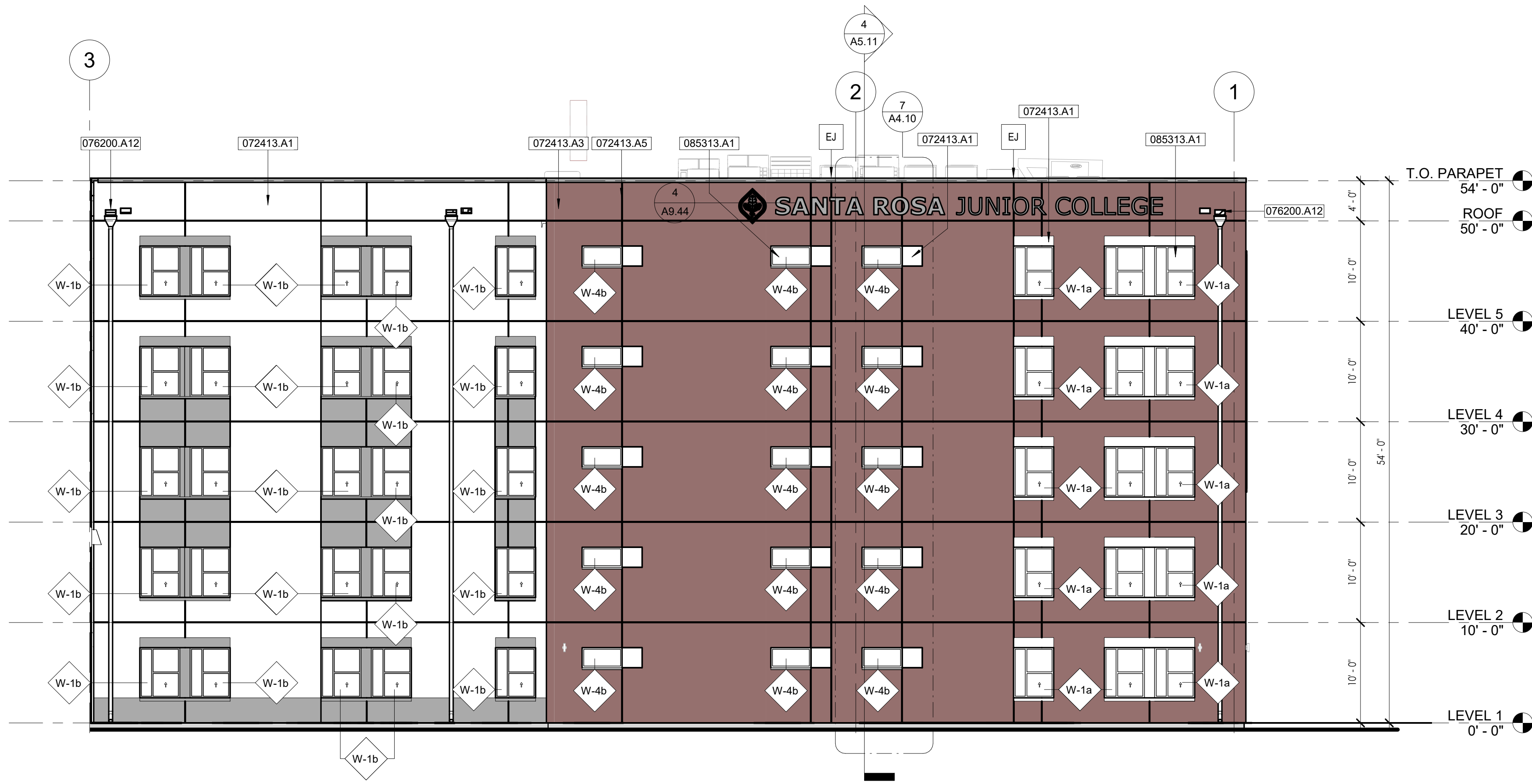
SOUTH WING - NORTH ELEVATION SCALE 1/8" = 1'-0" 1
