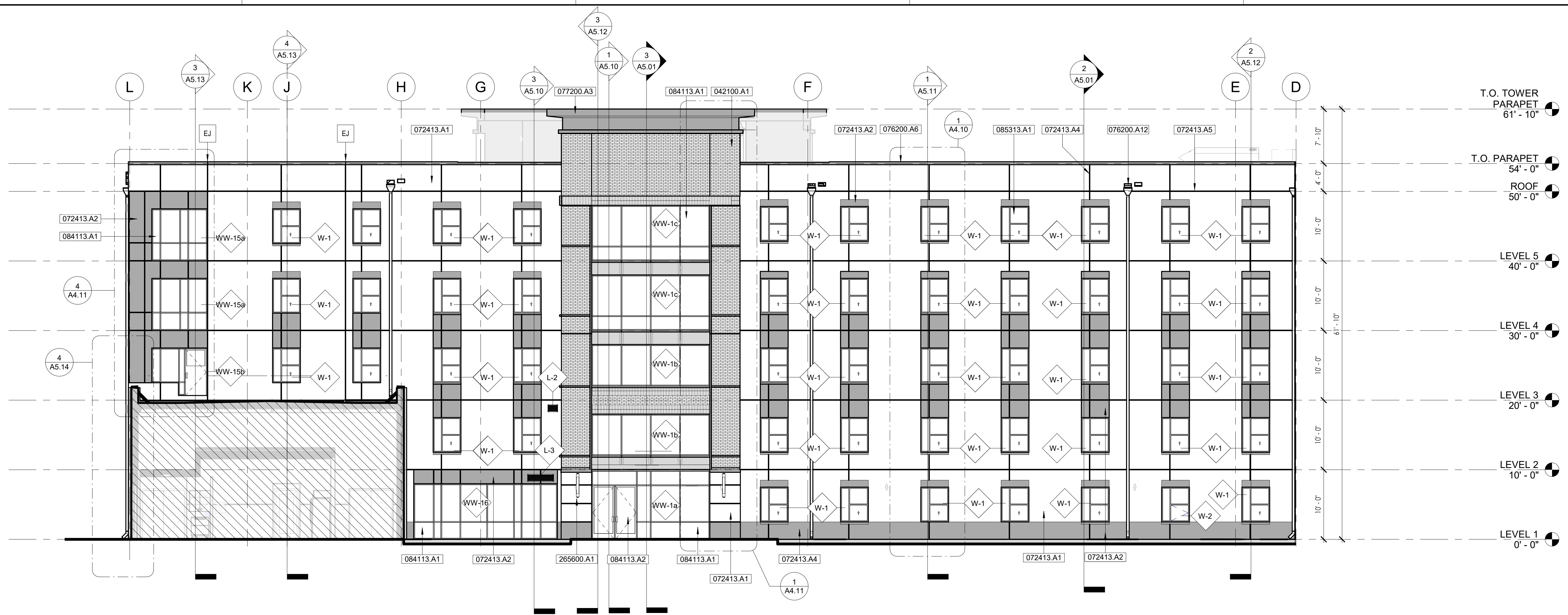
MAIN ENTRY/SOUTH WING - EAST ELEVATION SCALE 1/8" = 1'-0" 1
