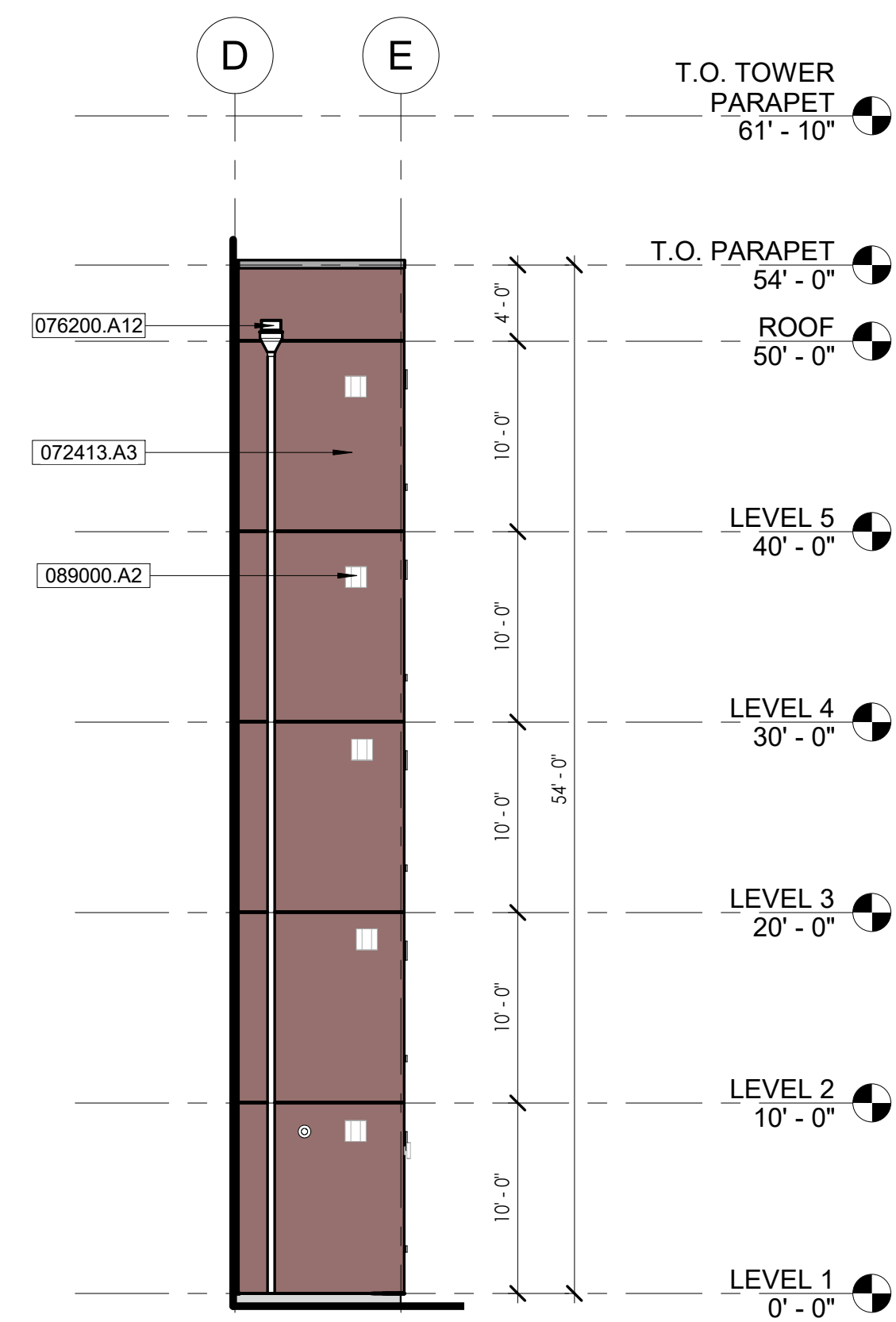
NORTH WING - RETURN ELEVATION - WEST ELEVATION SCALE 1/8" = 1'-0" 3
