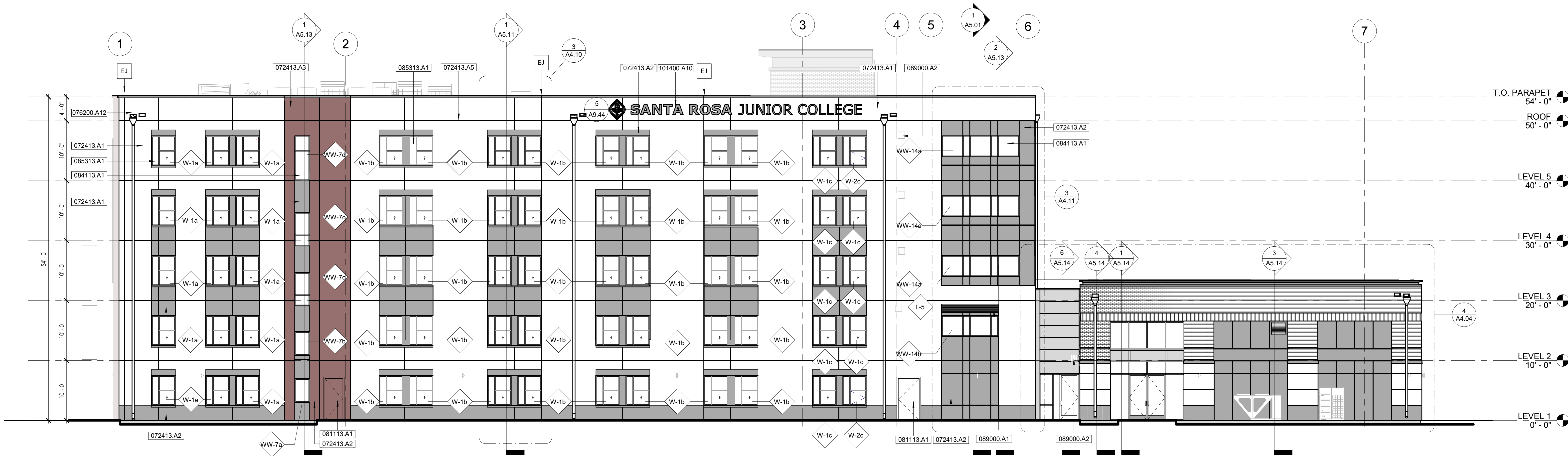
SOUTH WING - SOUTH ELEVATION SCALE 1/8" = 1'-0" 3
