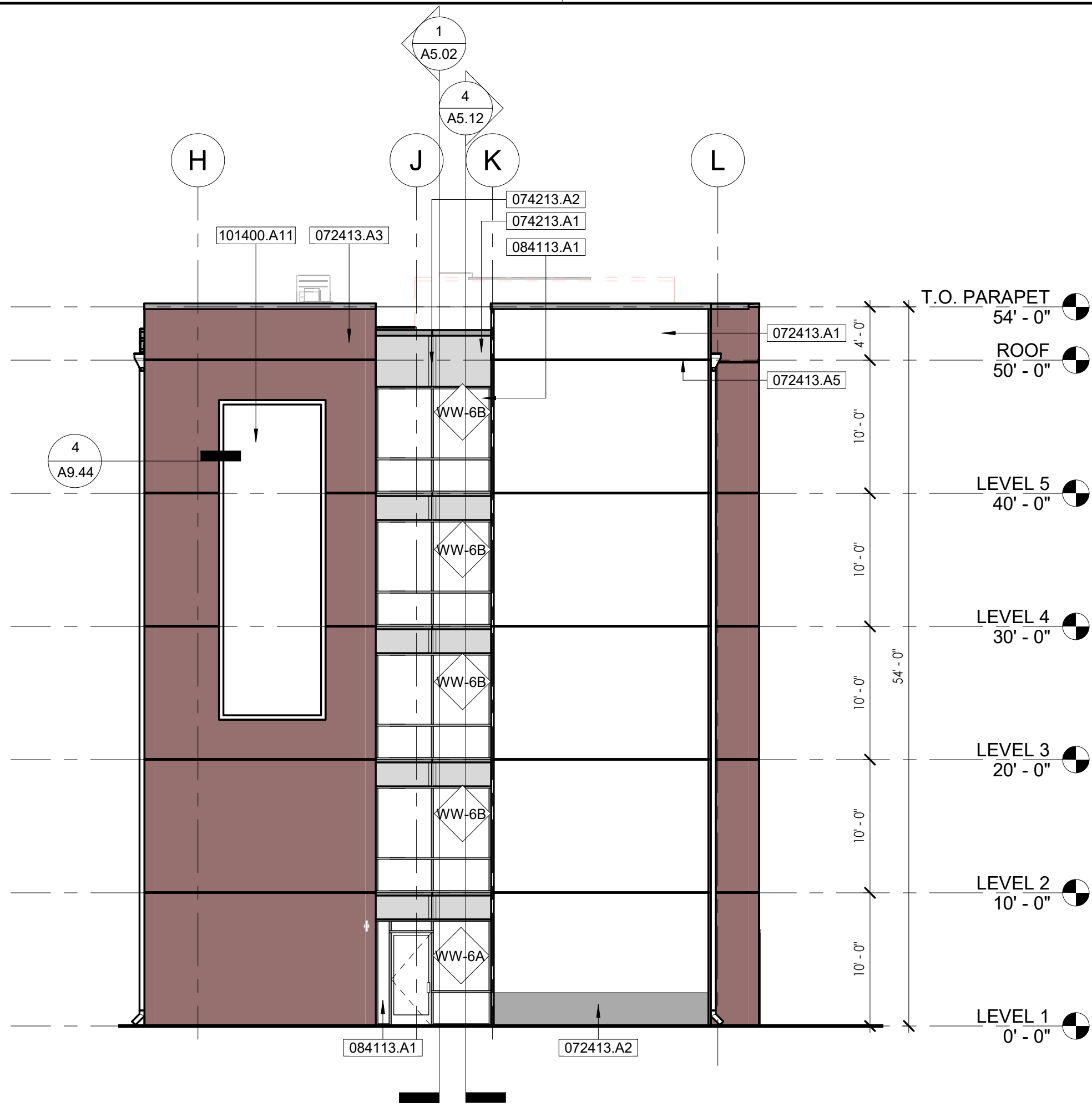
SOUTH WING - WEST ELEVATION SCALE 1/8" = 1'-0" 2
