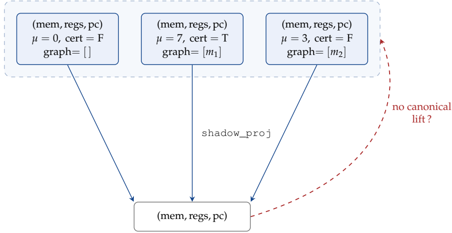
Figure 2: The directional structural theorem. Every Thiele state has a single canonical projection down via shadow_proj (degenerate_projection_theorem in coq/kernel/foundation/TuringClassicalEmbedding.v ). The classical state has multiple Thiele preimages and no canonical lift back (fiber_has_two_preimages in coq/kernel/witness/BlindnessRepresentation.v ). One direction is a function; the other is not.
