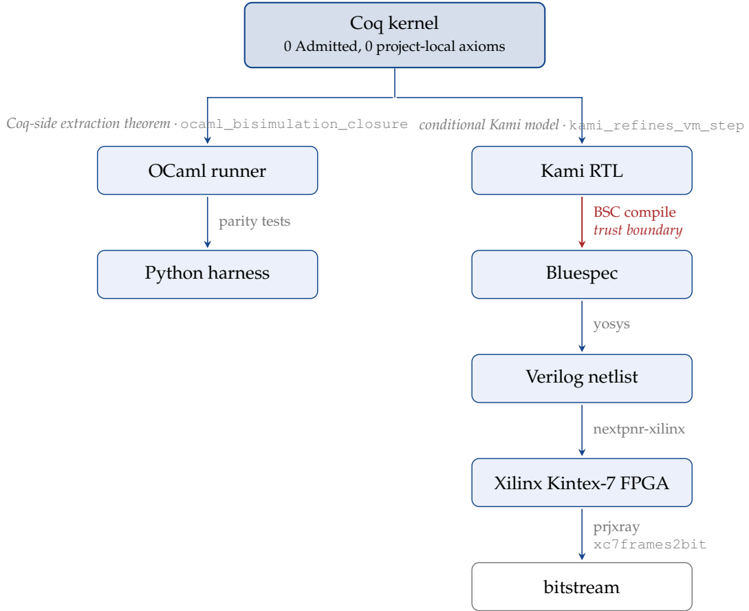
Figure 5: The three-layer realisation. The Coq kernel is the source of truth; the left branch is the runnable-binary path, the right branch is the silicon path. Blue arrows are either conditional Coq-model correspondences (with the theorem named on the edge) or empirical tests. The red and downstream tool arrows are translation/tool trust boundaries unless a separate theorem or artifact says otherwise; no single end-to-end RTL/bitstream bisimulation is claimed.
