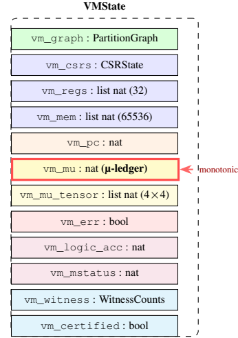
Figure 3.2: The VMState record: a complete, immutable snapshot of machine state. The \mu -ledger (highlighted) never decreases across transitions.
