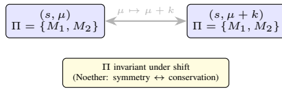
Figure 3.9: Gauge symmetry: shifting \mu by a constant k preserves partition structure. Only \mu differences (costs) are physically meaningful. This is the computational analog of Noether's theorem.
