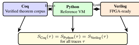
Figure 4.8: Chapter 4 summary: one Coq specification with two derived execution backends, bound by observable comparison gates.
