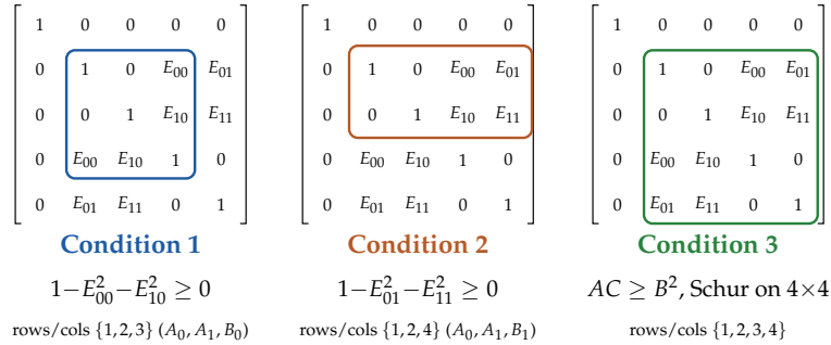
Figure 7: The 5 \times 5 zero-marginal NPA moment matrix shown three times, each copy highlighting one principal submatrix whose PSD condition gives one column-contractivity condition. Two come from 3 \times 3 principal-submatrix determinants; the third comes from the Schur complement of the 4 \times 4 block. All three follow from PSD of the parent matrix. Panel 2's \{1, 2, 4\} submatrix is non-contiguous, skipping row and column 3, so its highlight marks the band of rows the condition constrains rather than the exact cells; panels 1 and 3 are contiguous and highlighted exactly.
