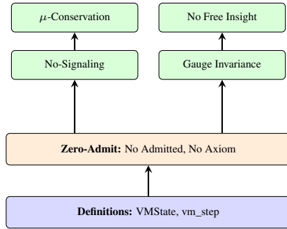
Figure 5.1: Chapter 5 verification pyramid. Foundational definitions support the zero-admit standard, which enables machine-checked proofs of the four core theorems.
