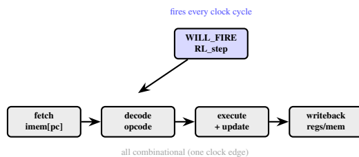
Figure 4.4: Single-rule execution model: the Kami-generated hardware performs fetch, decode, execute, and writeback combinational within one clock edge. No multi-cycle FSM pipeline.
