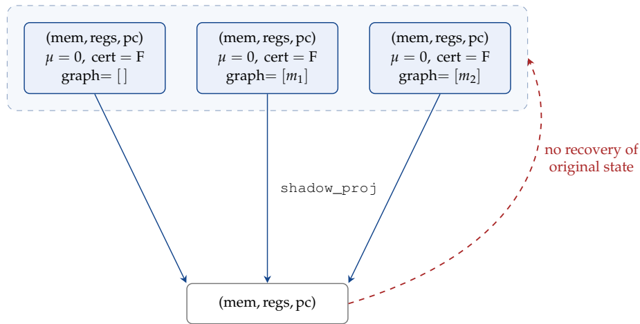
Figure 2: Different states, same view. When more than one state sits behind a view, no function of the view gets every original back. You can pick default values to fill the gaps. The defaults don't recover what was really there. Some kept fields are left out of the drawing so it stays readable.
