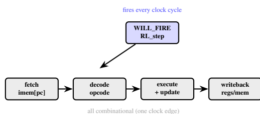
Figure 4.4: Single-rule execution model: the Kami-generated hardware performs fetch, decode, execute, and writeback combinationally within one clock edge. No multi-cycle FSM pipeline.
