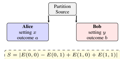
Figure 6.3: CHSH Bell test: Alice and Bob receive correlated partition states and make independent measurements.
