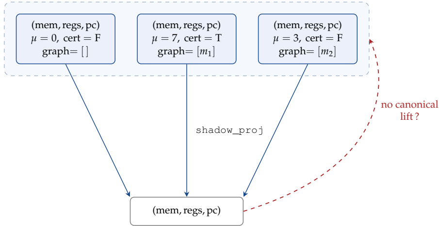
Figure 2: The directional structural theorem. Every Thiele state has a single canonical projection down via \text{shadow\_proj} ( \text{degenerate\_projection\_theorem} ). The classical state has multiple Thiele preimages and no canonical lift back ( \text{fiber\_has\_two\_preimages} ). One direction is a function; the other is not.
