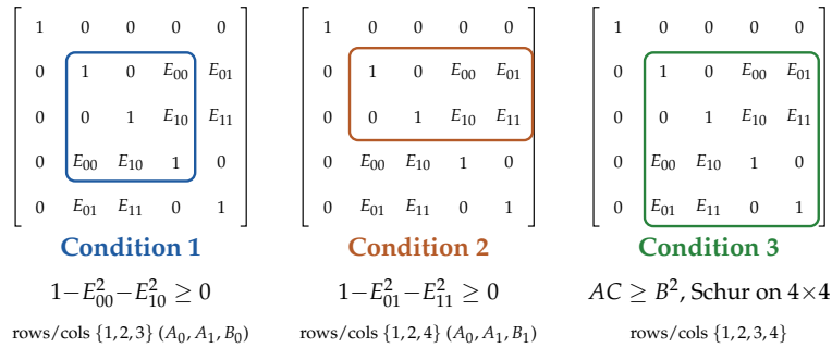
Figure 7: The 5 \times 5 zero-marginal NPA moment matrix shown three times, each copy highlighting one principal submatrix whose PSD condition gives one column-contractivity condition. Two come from 3 \times 3 principal-submatrix determinants; the third comes from the Schur complement of the 4 \times 4 block. All three follow from PSD of the parent matrix. Panel 2's \{1, 2, 4\} submatrix is non-contiguous, skipping row and column 3, so its highlight marks the band of rows the condition constrains rather than the exact cells; panels 1 and 3 are contiguous and highlighted exactly.
