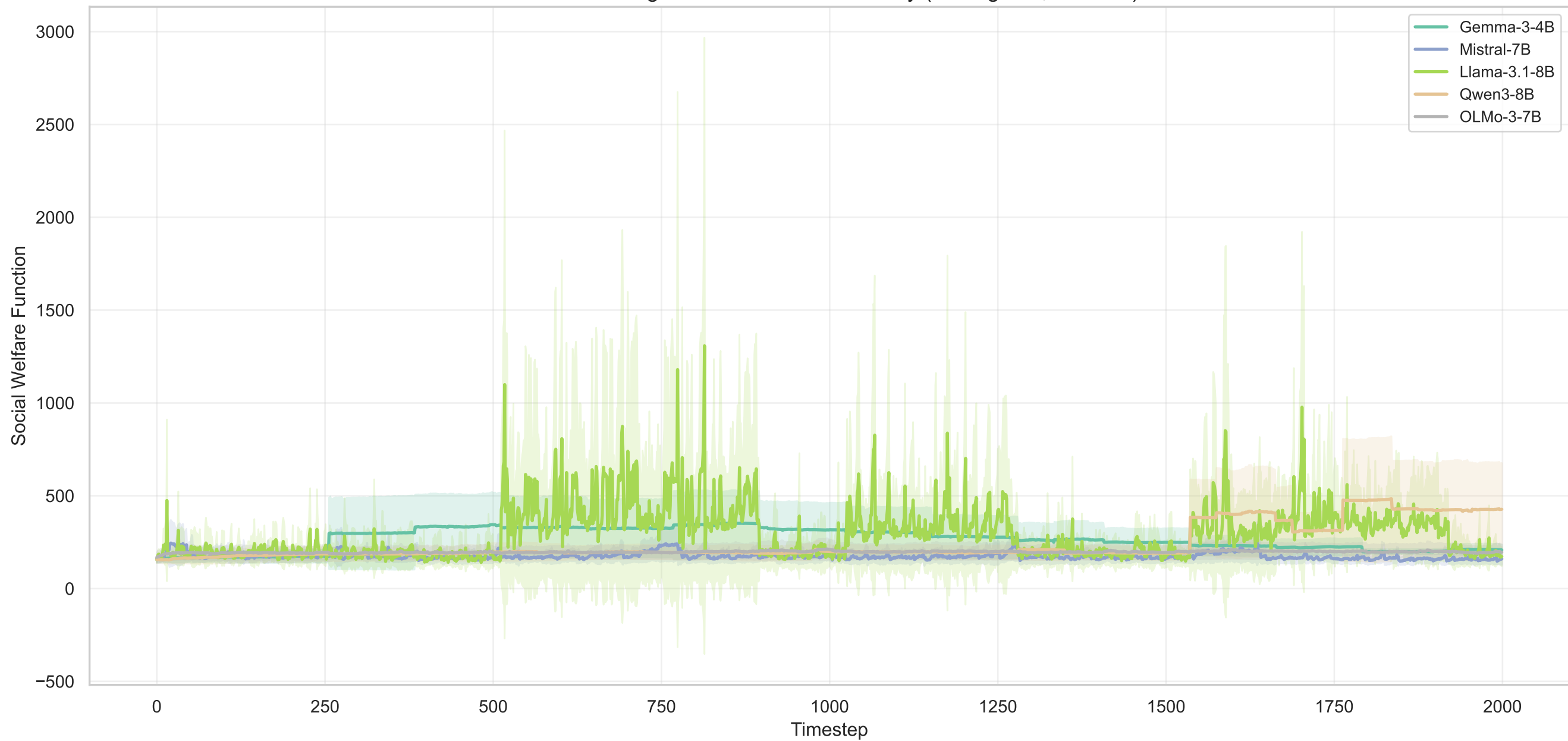
SWF Convergence: Bounded Rationality (100 agents, 3 seeds)
