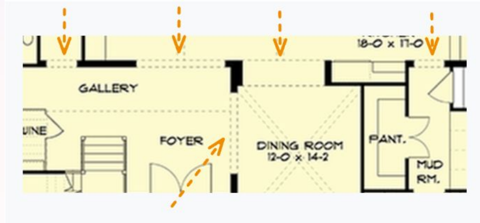
Openings shown by two parallel dotted lines between two walls
