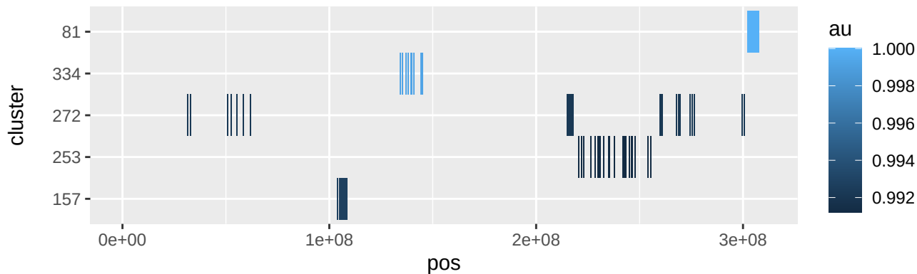
single/uncentered, 5–300 blocks P > 0.99 1000 boots
