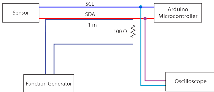
Figure 1: Wiring schematic of the project experimental setup. A function generator outputs a sinusoidal signal through a wire connected by a 100Ω resistor. The signal line is routed adjacent to the sensor's data line to induce electromagnetic coupling. The microcontroller and sensor communicated over the SDA line close to the wire and an SCL far from it. The Arduino communicates to and is powered by the computer via USB.
