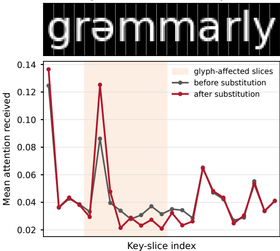
(a) Average attention received by each slice
