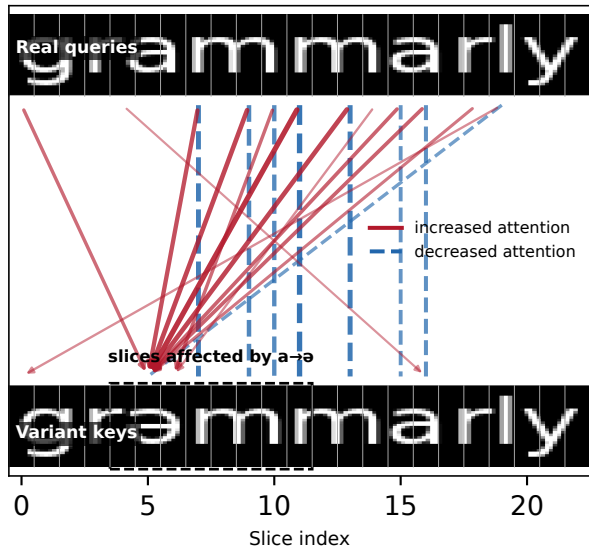
(b) Cross-attention: adaptive routing
