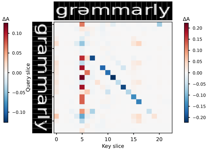
(b) B1: real \rightarrow variant
