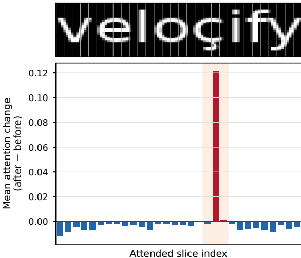
(a) Substitution-induced attention change by slice
