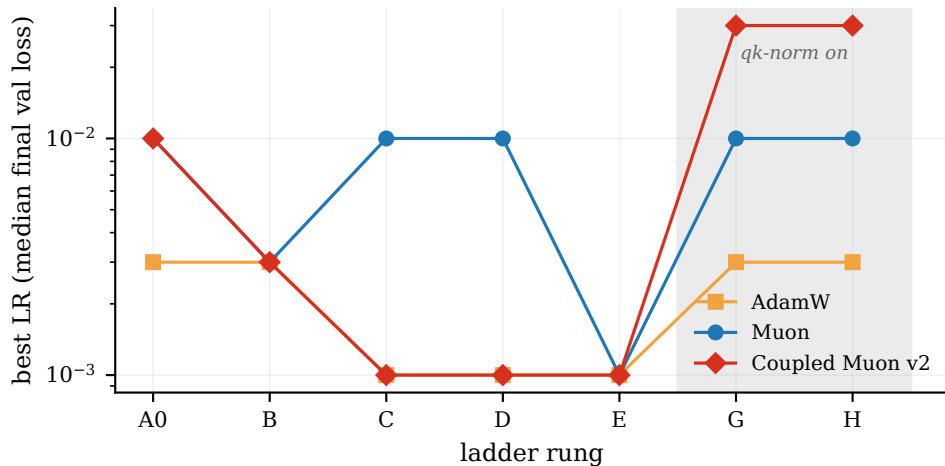
Best LR per (rung, optimizer): operating point drift between non-QK-Norm and QK-Norm rungs
