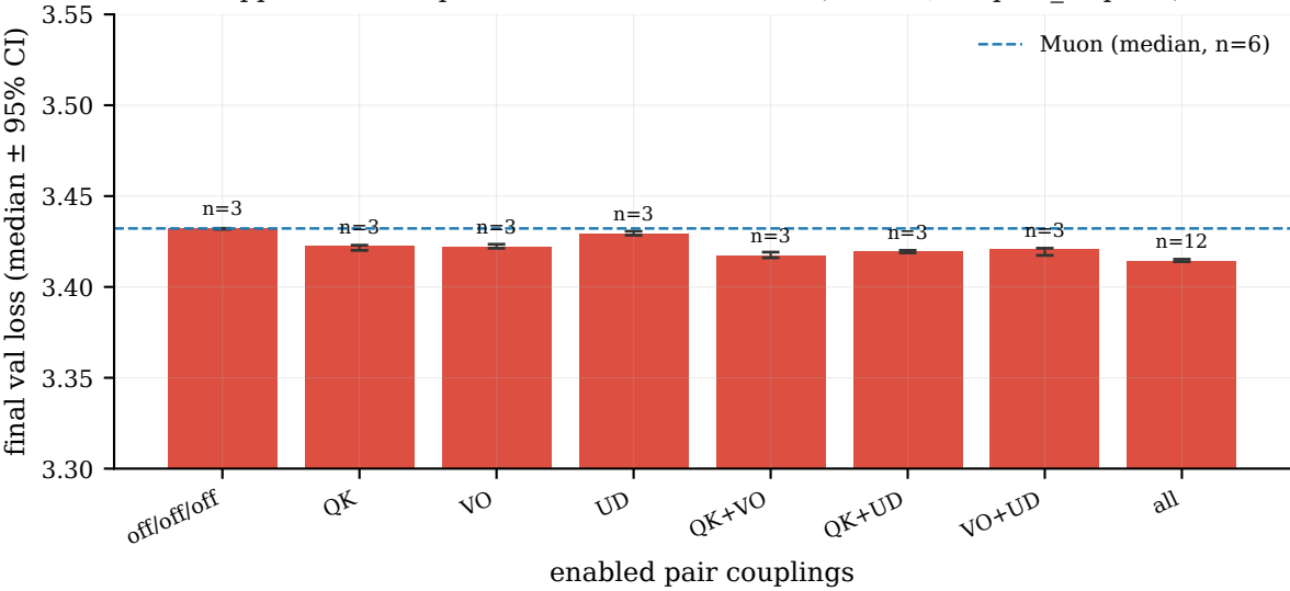
App. B.3 — Full pair-factorial ablation at A0 (lr=3e-3, coupled_steps=4)
