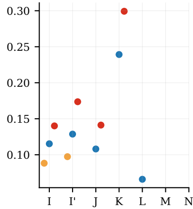
grad-norm var
