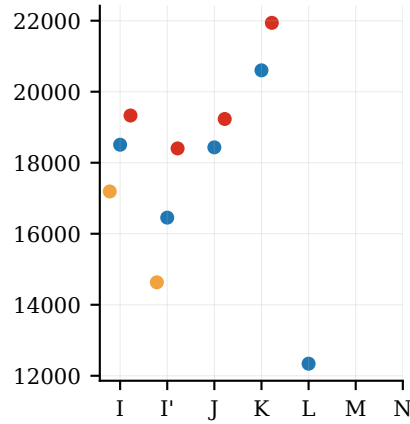
runtime (s)
