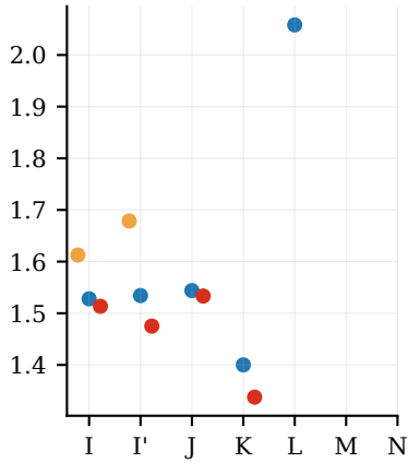
router entropy
