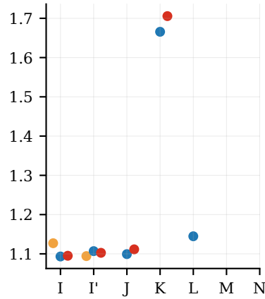
load imbalance
