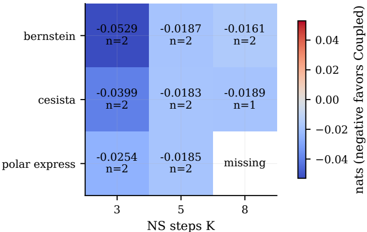
NS-policy sweep: Coupled - Muon final val loss
