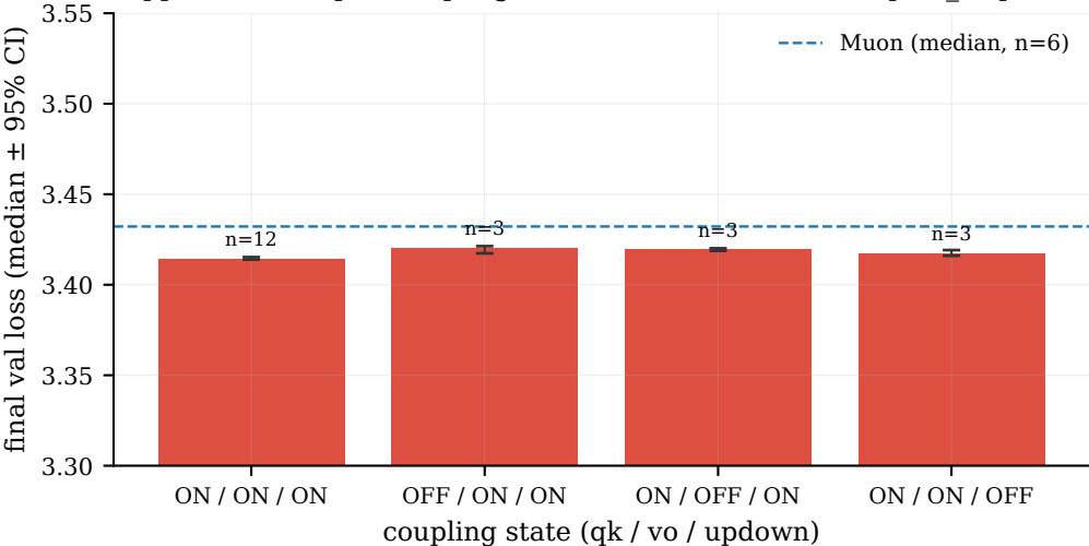
App. B.3 — Per-pair coupling ablation at A0 (lr=3e-3, coupled_steps=4)
