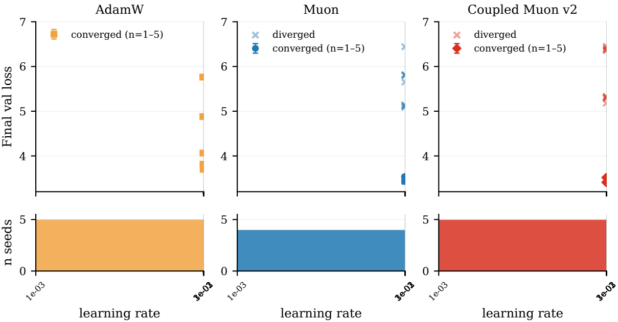
Stage 1 (A0 LLaMA-60M): LR sensitivity and divergence count per optimizer
