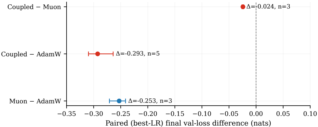
Stage 1 (A0): paired-bootstrap 95% CIs at each arm's best LR
