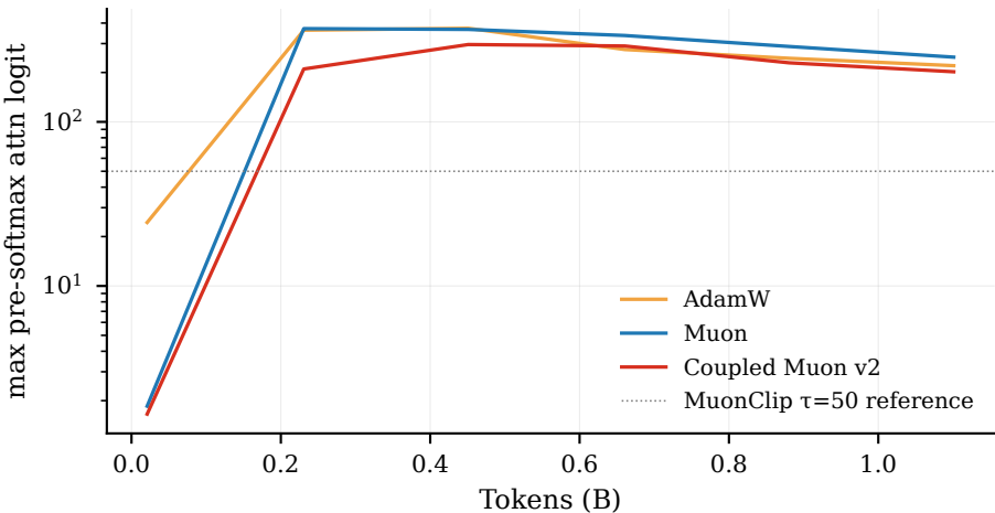
Stage 1 (A0): global-max attention logit trace (MuonClip stability)
