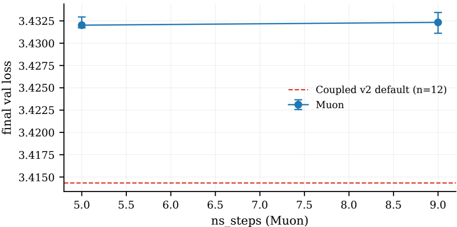
App. B.5 — Muon NS budget control (does extra NS alone match coupling?)
