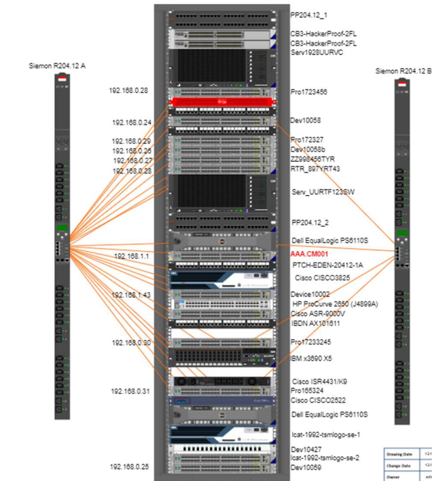
Physical topology diagrams
