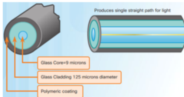
Single-Mode Fiber
