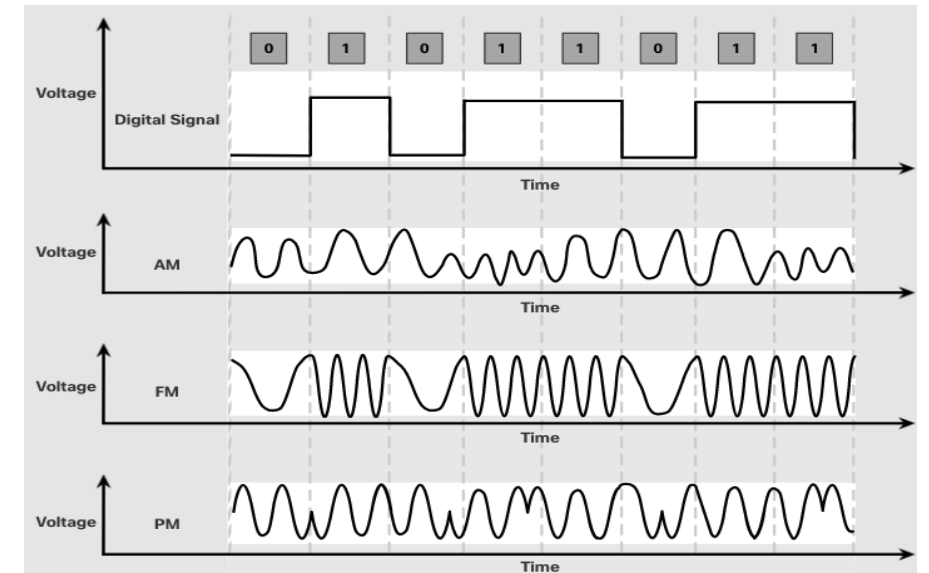
Microwave Signals Over Wireless
