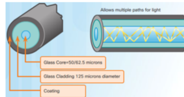
Multimode Fiber
